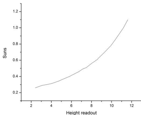
Typical attenuation behavior of the 11002 SunLite™ Solar Simulator using the model 15279 option.
